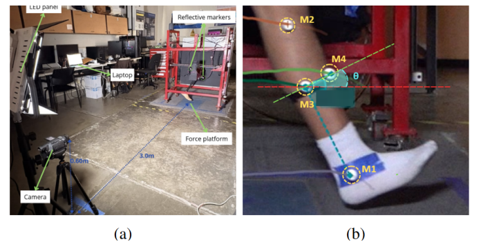
Fig. 4. (a) Experimental setup for kinematic and kinetic data acquisition, (b) Placement of markers M1–M4 on the reference subject and definition of the tibial-segment inclination angle \theta .
